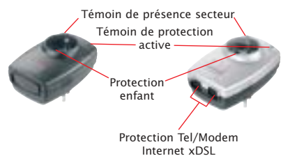
Protection Box 1
